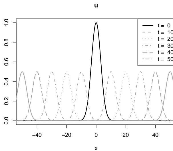
Figure 3: The 1-D wave equation; black = initial condition; grey: several time lines
